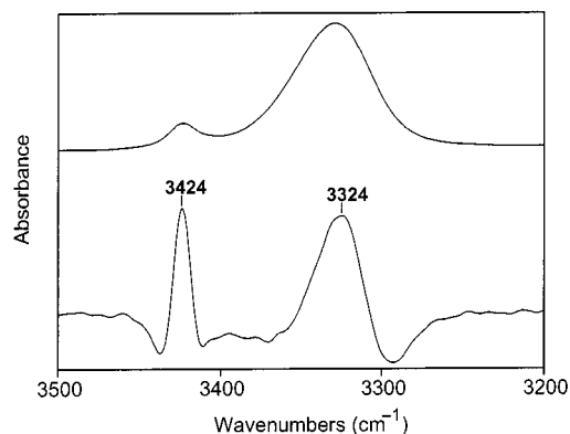
Figure 9. FT-IR absorption and inverted second derivative spectrum of Boc-( S )-[20-C-6]-Bip-(Aib) 6 -OrBu in CDCl 3 solution; peptide concentration 1 mM
