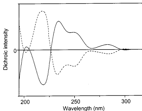
Figure 11. CD spectra of Boc-( S )-[20-C-6]-Bip-(Aib) 6 -OrBu VI (-----) and the model compound Boc-( R )-[20-C-6]-Bip-OH Ic (----) in MeOH solution
