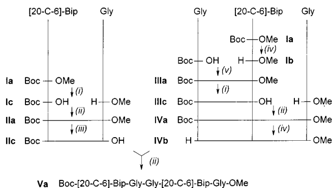
Figure 8. Solution synthesis of peptides I – V : (i) 1 N NaOH, MeOH, 50 °C, 2 h; (ii) EDC, HOBt; (iii) 1 N NaOH, MeOH, room temp., 2 h; (iv) TFA/CH 2 Cl 2 (1:3), room temp., 2.5 h; (v) (1) Boc-Gly-OH (2 equiv.), EDC, CH 3 CN, room temp., 1 h; (2) H-[20-C-6]-Bip-OMe
