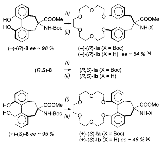
Figure 6. Synthesis of racemic and chirally resolved Boc-[20-C-6]-Bip-OMe ( 1a ) and H-[20-C-6]-Bip-OMe ( 1b ): (i) Cs 2 CO 3 , TsO-CH 2 -(CH 2 -O-CH 2 ) 4 -CH 2 -OTs, DMF, 60 °C; (ii) TFA/CH 2 Cl 2 (1:3), room temp.; 19 F enantiomeric excess determined by 19 F NMR of the corresponding Mosher amide (see text and Exp. Sect.)
