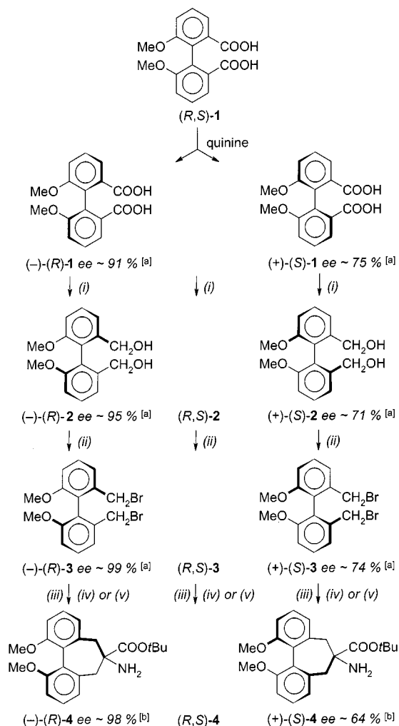
Figure 2. Synthesis of racemic and chiral resolved H-[MeO] 2 -Bip-OrBu ( 4 ): (i) BH 3 , THF, 0 to 25 °C, 5 h; (ii) PBr 3 , toluene, 0 to 45 °C; (iii) (4-chlorobenzylidene)glycine tert -butyl ester, KOH powder, K 2 CO 3 , CH 2 Cl 2 , room temp.; (iv) NH 2 OH·HCl, AcONa, 95% EtOH, room temp.; (v) 0.5 M citric acid, THF, room temp.; [a] enantiomeric excess (optical purity) determined by comparison of the optical rotation with the maximum value from literature (see text and Exp. Sect.); [b] determined by 19 F NMR of the corresponding Mosher amide (see text and Exp. Sect.)
