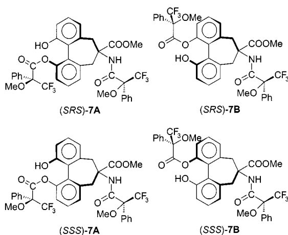
Figure 5. Chemical structures of the four diastereoisomeric Mosher amides/half phenyl esters 7A and 7B ; note: position of the phenyl ester function in 7A and 7B has been arbitrarily assigned
