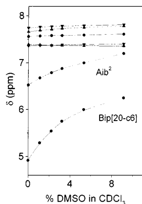
Figure 10. Plot of NH chemical shifts in the 1 H NMR spectrum of Boc-( S )-[20-C-6]-Bip-(Aib) 6 -OrBu as a function of increasing percentages of DMSO (v/v) added to the CDCl 3 solution; peptide concentration 1 mM
