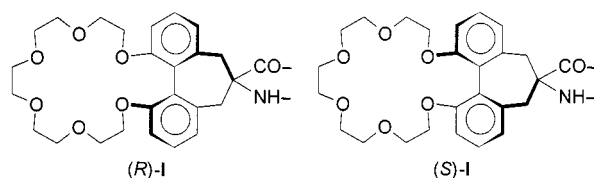
Figure 1. Chemical structure of the enantiomeric crown-carrier, axially dissymmetric, C^{\alpha,\alpha} -disubstituted glycol residue [20-C-6]-Bip ( R )- I and ( S )- I
