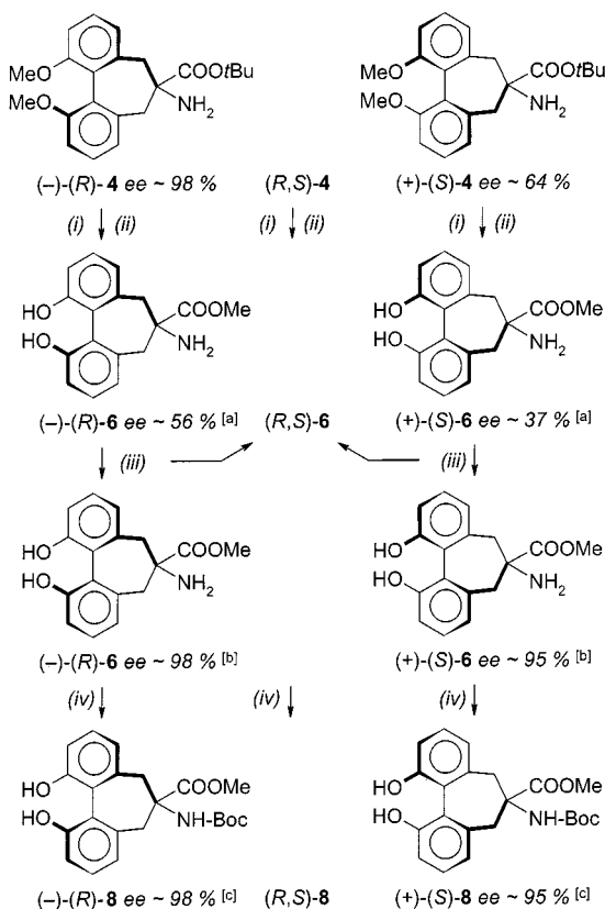
Figure 4. Synthesis of racemic and chirally resolved H-[HO] 2 -Bip-OMe ( 6 ) and Boc-[HO] 2 -Bip-OMe ( 8 ); (i) BBr 3 , CH 2 Cl 2 , room temp.; (ii) MeOH, 98% H 2 SO 4 (cat.), reflux; (iii) fractional crystallization of ( R,S )- 6 ; (iv) Boc 2 O, CH 3 CN, room temp. or 75 °C (for racemic); [a] enantiomeric excess (optical purity), determined by comparison of the optical rotation with the calculated maximum value (see text and Exp. Sect.); [b] determined by 19 F NMR of the corresponding Mosher's amides/half phenyl ester isomers (see text and Exp. Sect.); [c] assumed (see text)
