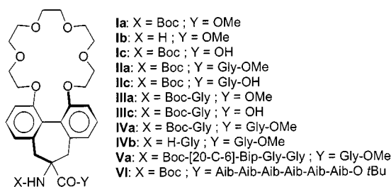
Figure 7. Chemical structures of the peptides I – VI based on the [20-C-6]-Bip residue
