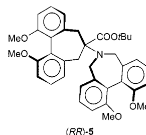
Figure 3. Chemical structure of the side product ( RR )- 5
